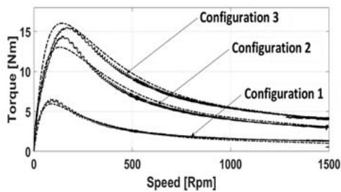
7b Torque curves at 6A
