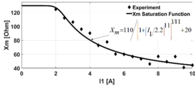
Fig. 4. Mutual reactance at different levels of current .
